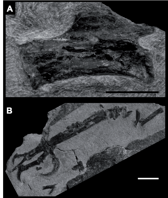
Fig. 4. Archosaurian remains. A, posterior caudal vertebra of a possible coelurosaurian theropod in lateral view; B, left articulated foot of the enantiornithine bird Intiornis inexpectatus . Scale bar 10 mm.
