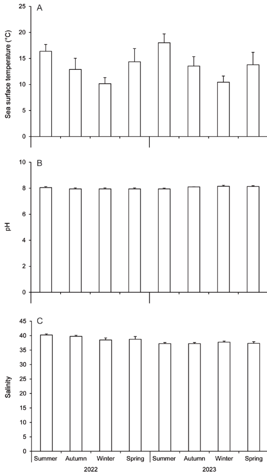
Fig. 4. Seasonal environmental variables (A) Mean sea surface temperature ( ^{\circ}\text{C} \pm \text{SD} ) recorded by ElectricBlue loggers; (B) Mean pH ( \pm \text{SD} ), and (C) Mean salinity ( \pm \text{SD} ) over the two years sampled in the intertidal boulder fields of Puerto Lobos Protected Natural Area.
