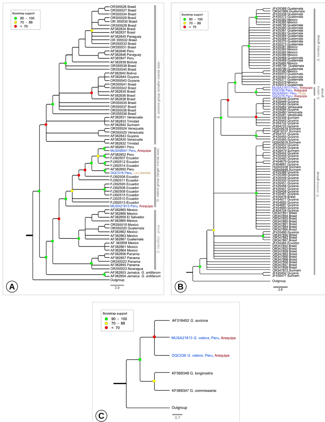
Fig. 3. Phylogenetic relationships of Glossophaga species inferred by Bayesian inference based on: A. Cyt B with 775 bp. B. COI of 509 bp. C. RAG2 with 479 bp.
