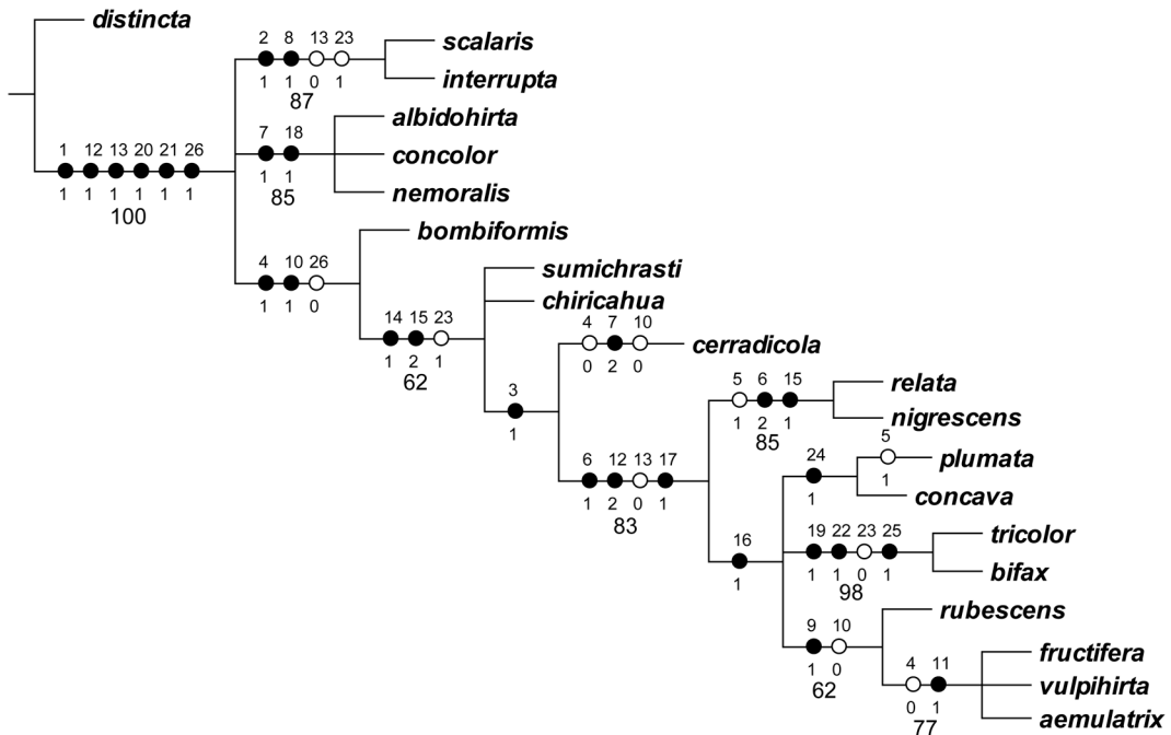
Fig. 2. Strict consensus tree depicting relationships among species of Ptilothrix based on morphological characters. Black hash marks indicate nonhomoplastic changes. Large numbers below branches indicate bootstrap values.
